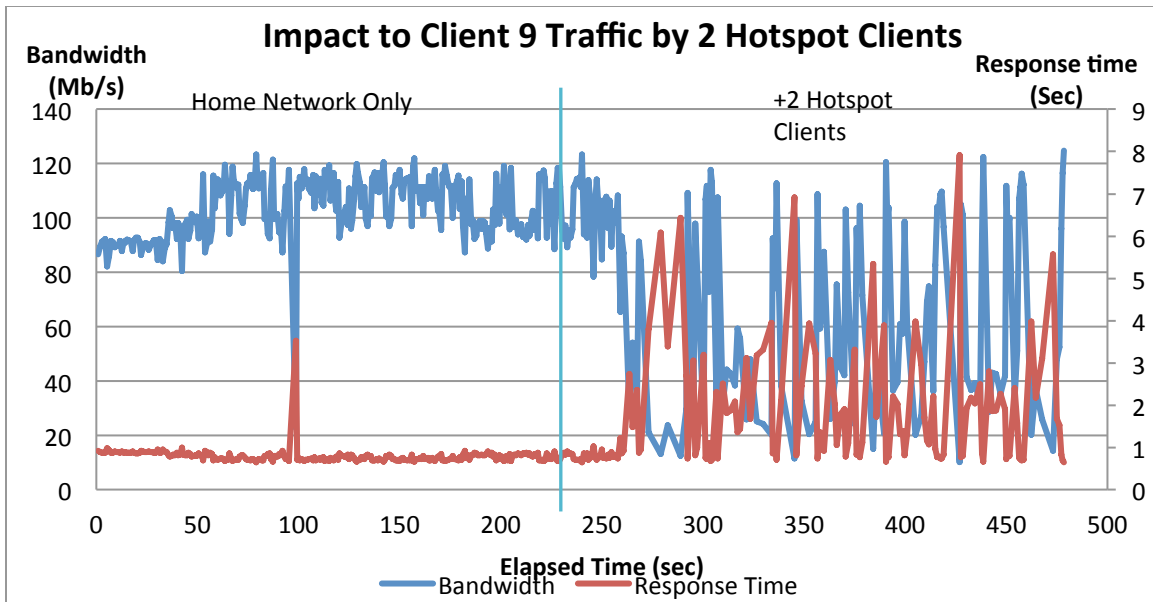
Figure 13: Client 9 Bandwidth and Response Time (Hotspot Traffic Starts 4 Minutes into the Test)
