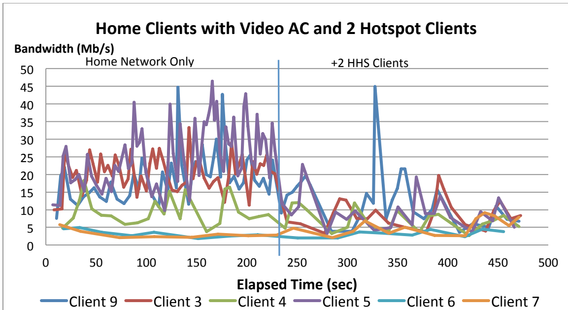
Figure 14: 6 Home Clients Bandwidth (Hotspot Traffic Starts 4 Minutes into the Test)
